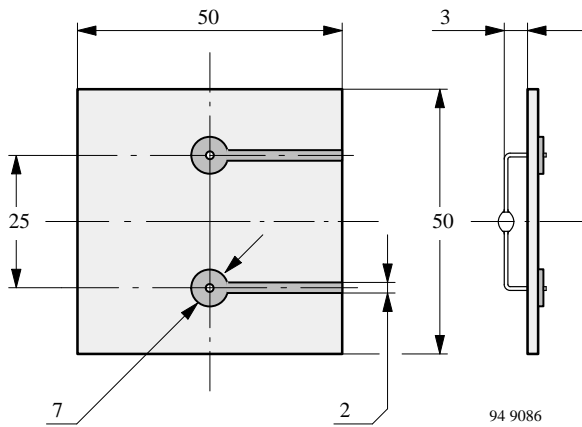
Figure 1 : Epoxy glass hard tissue, board thickness 1.5 mm, R_{thJA} \leq 110 \text{ K/W}
